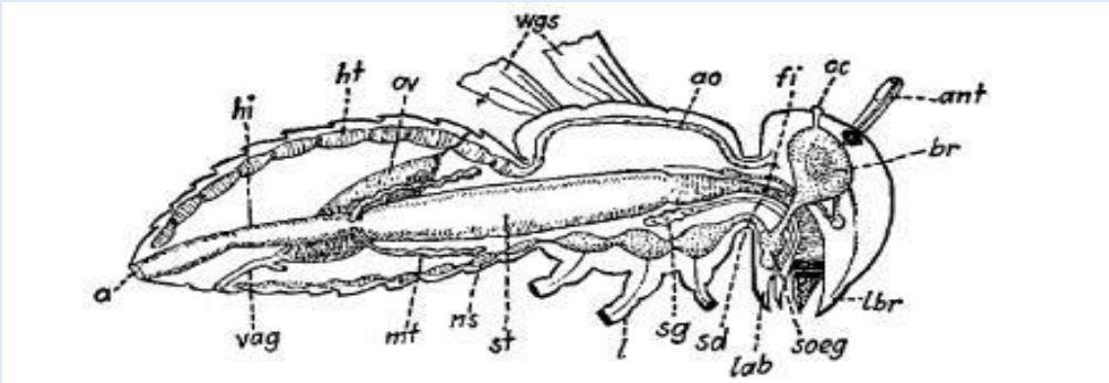
FIG. 23.—Diagrammatic longitudinal section of an insect to show the arrangement of the internal organs: a, anus; ant, antenna; ao, aorta; br, brain; fi, fore intestine; hi, hind intestine; ht, heart; l, leg; lab, labium; lbr, labrum; mt, Malpighian tube; ns, nervous system; oc, ocellus; ov, ovary; sd, salivary duct; sg, salivary gland; soeg, subesophageal ganglion; st, stomach (mid intestine); vag, vagina; wgs, wings. (After Berlese.)
