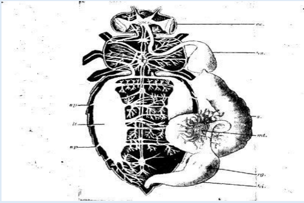
FIG. 25.—Internal anatomy of the honeybee showing alimentary canal, tracheal and nervous systems: ce. , compound eye; hi. , hind intestine; ha. , honey stomach; lt. , lateral trachea (enlarged); mt. , Malpighian tubes; rg. , rectal glands; s. , stomach; sp. , spiracles. (Modified from Leuckart's Wandtafel .)
