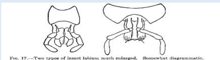
FIG. 17.—Two types of insect labium much enlarged. Somewhat diagrammatic.
