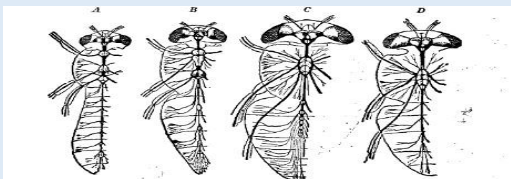
FIG. 29.—Diagram showing various degrees of concentration forward of the nervous system of four species of flies: A, Chironomus plumosus , little concentrated; B, Empis stereocera ; C, Tabanus bovinus ; D, Sarcophaga carnaria , most concentrated. (After Brandt, from Lang's Lehrbuch .)
