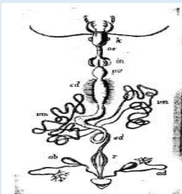
FIG. 24.—Alimentary canal of a carnivorous beetle: ad. , anal glands; cd. , stomach; ed. , hind intestine; in. , crop; k. , head and mouth-parts; oe. , esophagus; pv. , proventriculus; r. , rectum; em. , Malpighian tubes. (Modified from Lang's Lehrbuch .)
