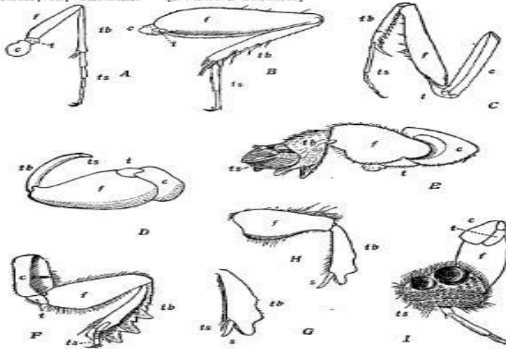
FIG. 18.—Different forms of insect legs: A , Cicindela sexguttata Fab. (beetle); B , Nemobius fasciatus De G. (cricket) hind leg; C , Stagmomantis carolina L. (mantis) foreleg; D , Polocoris femoratus P. B. (carnivorous bug) foreleg; E , Gryllotalpa hexadactyla Perty (mole cricket) foreleg; F , Canthion laxis Dru. (a digging beetle) foreleg; G , Phanæus carnifex L. (a digging beetle) fore tibia and tarsus of female; H , same, fore tibia of male; I , Dytiscus fasciventris Say, male (water beetle) foreleg. c , coxa; f , femur; s , spine; t , trochanter; tb , tibia; ts , tarsus. (From Folsom.)
